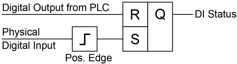
Figure 7: Input latch
