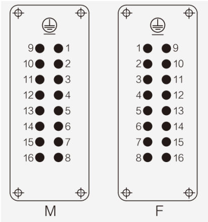
Pin assignment
