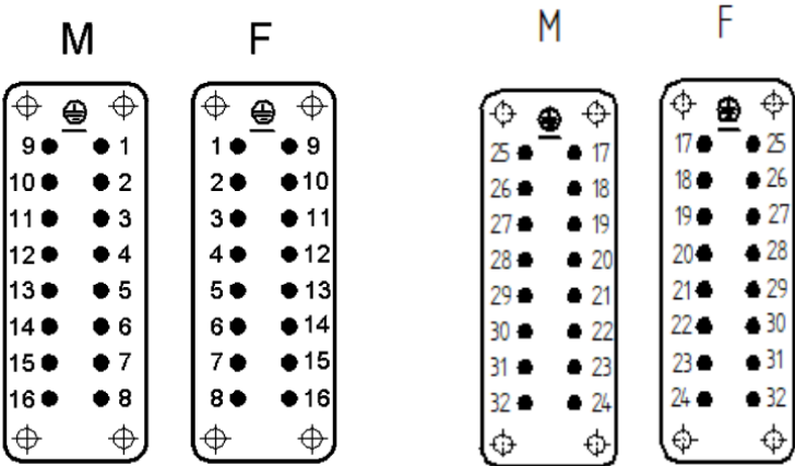
Pin assignment
