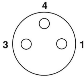
Pin assignment M8-jack, 3-pol, A-coding
