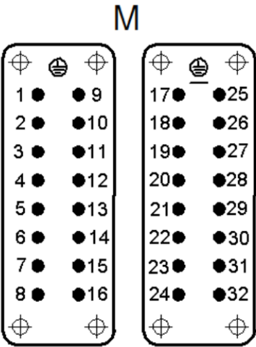
Pin assignment
