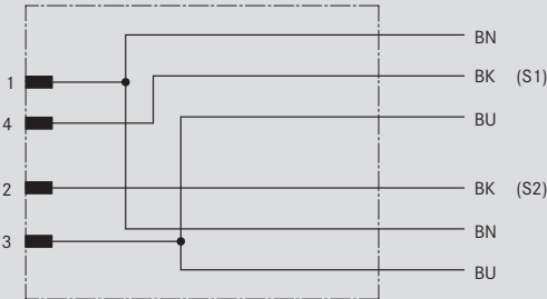
Y-distributor M12Y on free conductor end
