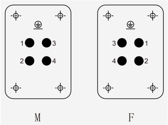
Pin assignment
