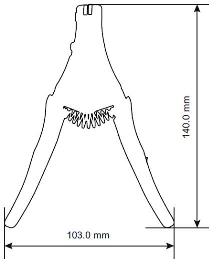
Dimensions cable stripper
